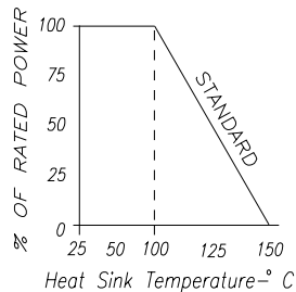
DERATING CURVE:
